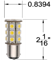
BA15d Double Contact D.C. Index Bayonet Base
